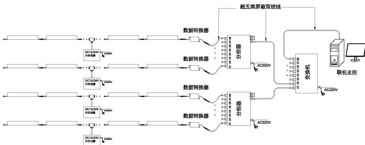
联机系统图 Online Controlling System Diagram
