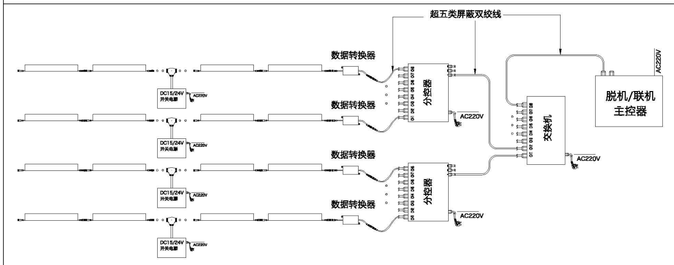
脱机系统图 Offline Controlling System Diagram
